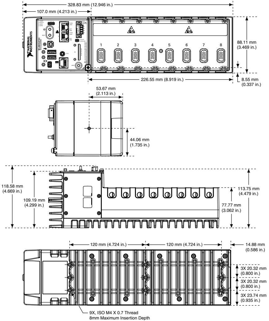
Figure 1. NI cDAQ-9133 Dimensions
