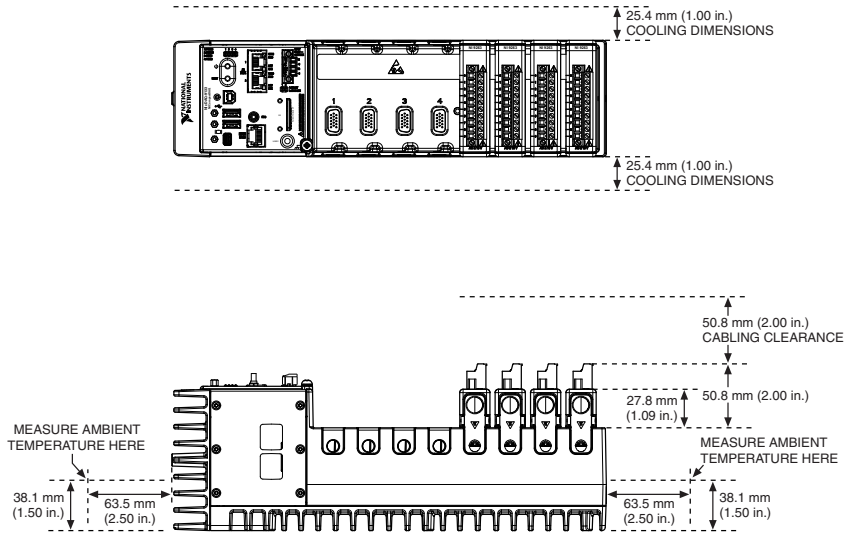
Figure 2. NI cDAQ-9133 Temperature, Cooling, and Cabling Dimensions
